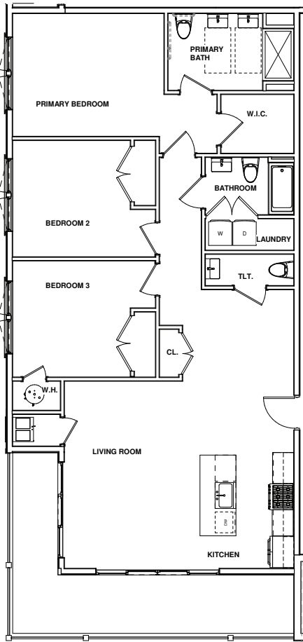
Plan 7 3 BR | 2.5 BA | 1,596 s.f. Including 252 s.f. deck
